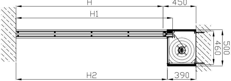
Type 1 housing.
