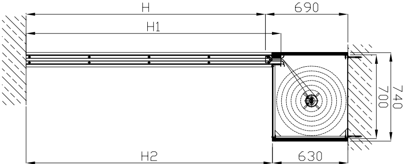
Type 4 housing.
