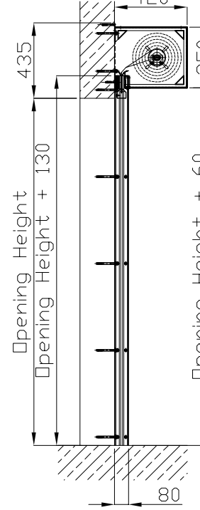
Type 4 housing.
