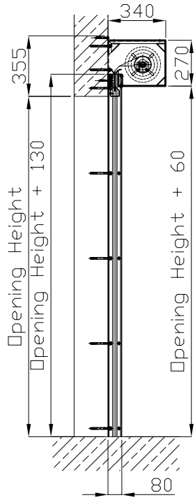
Type 2 housing.
