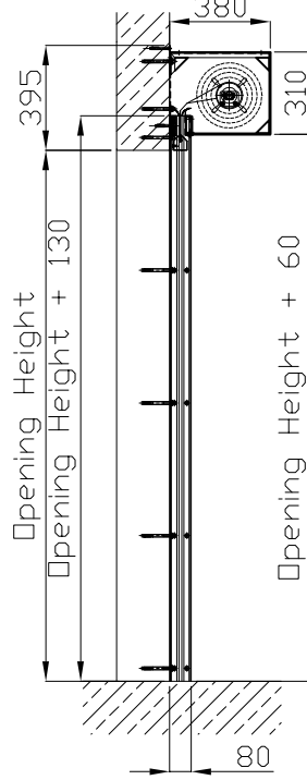
Type 3 housing.
