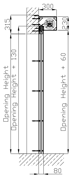
Type 1 housing.
