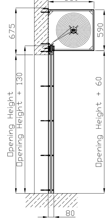
Type 10 housing.
