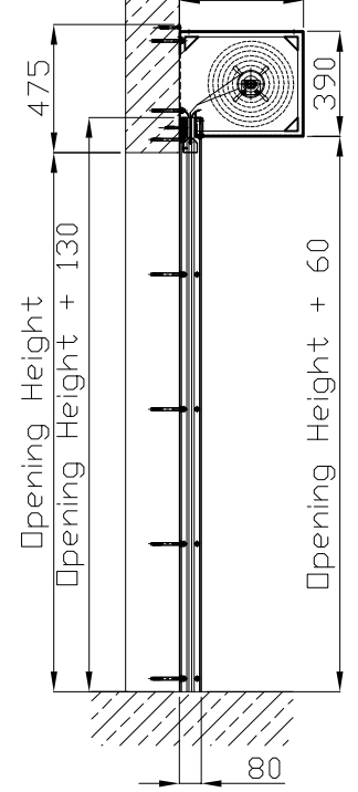
Type 5 housing.
