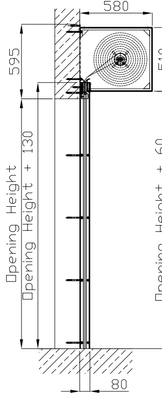
Type 8 housing.
