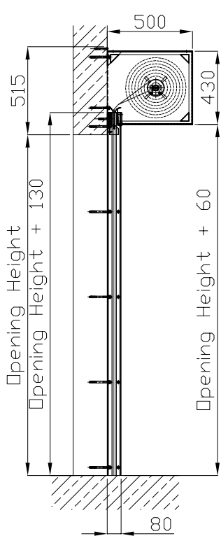
Type 6 housing.
