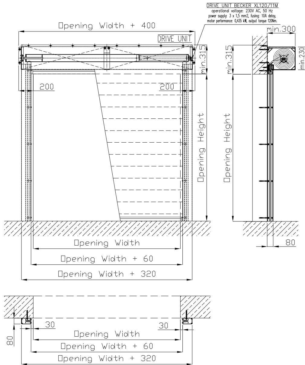
Type 2 housing.
