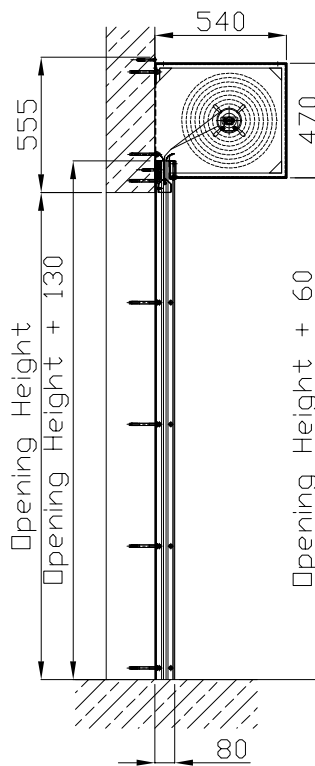
Type 7 housing.
